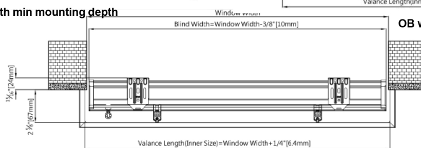
Semi-IB with shallow mounting holes
