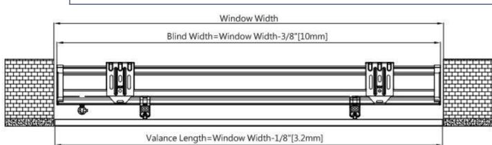
Fully IB with flush valance
