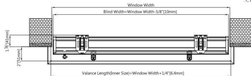
Semi-IB with min mounting depth
