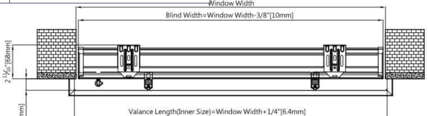
Semi-IB with bracket flush to wall
